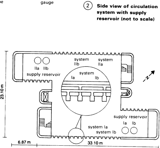
3 Water cooling scheme
